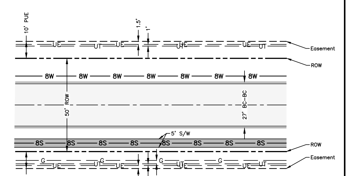
Typical Utility Layout Legend
